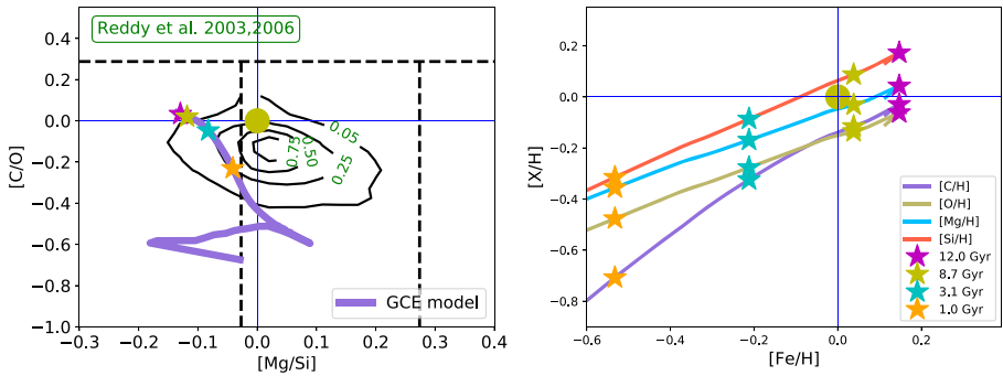
Fig. 2 Left Panel: stellar statistics distribution with respect to [C/O] and [Mg/Si] from observations [157, 158] and GCE models. The elemental ratios are reported in logarithmic notation, scaled to solar value. The Sun is reported as reference, with blue lines indicating the solar ratios. Dashed black lines indicate the element classification relevant for planet behavior according to [200]. GCE simulations are reported (magenta line), with reference time symbols at 1 Gyr, 3.1 Gyr, 8.2 Gyr (which corresponds to the age of the Sun) and 12 Gyr after the formation of the Milky Way (orange, cyan, yellow and magenta star, respectively). Right Panel: [C/H], [O/H], [Mg/H] and [Si/H] are reported with respect to [Fe/H] for the same GCE model reported in the left panel
